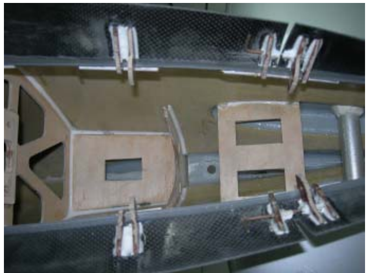
Inside view of hinges with plastic tube and steel pin
