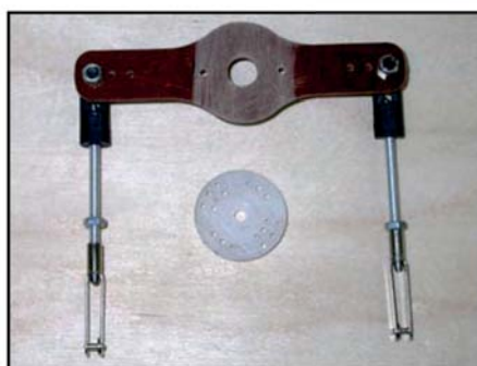
(below) The 4 phenolic rudder horns are glued and screwed onto standard 1" plastic servo discs.
