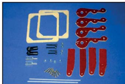
(above) The hardware & plywood servo hatch reinforcement parts for fitting the optional 3rd aileron servo are all included in the standard kit.
