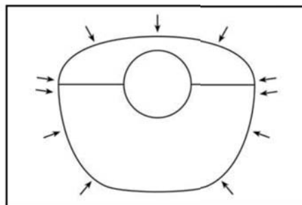
(above) The cowling is secured to the fuselage with 11 bolts, positioned as shown.
