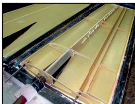
The internal structure of the Extra 260 wings, before the carbon rovings are added above & below the spar during the joining process.
