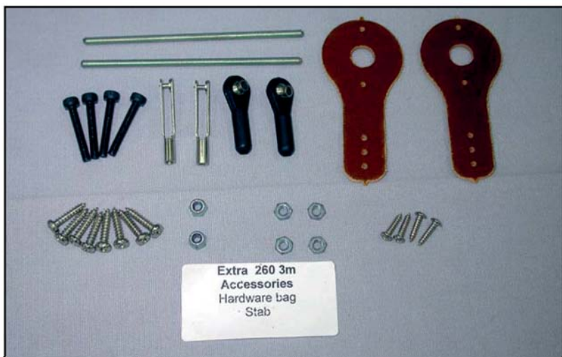
(above) Stab Hardware for each stab (2 sets included in kit)
