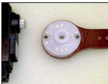
(above) The supplied phenolic servo arms are glued and screwed onto standard 1" plastic servo discs, but if using JR 8511/8611 servos you must use metal output arms or discs.
