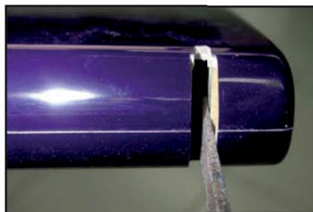
(below) If you want more elevator travel than the CNC milled slots in the elevator L.E will allow, you can extend them with a narrow file as shown here.
