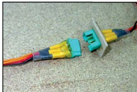
(above/below) We use these 6-pin Multiplex connectors for all the removable connections between wings/stabs and fuselage.
